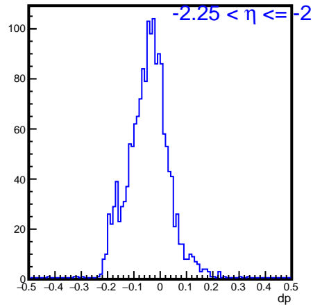
dp_eta_-2.250000_-2.000000
