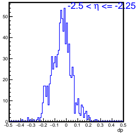
dp_eta_-2.500000_-2.250000
