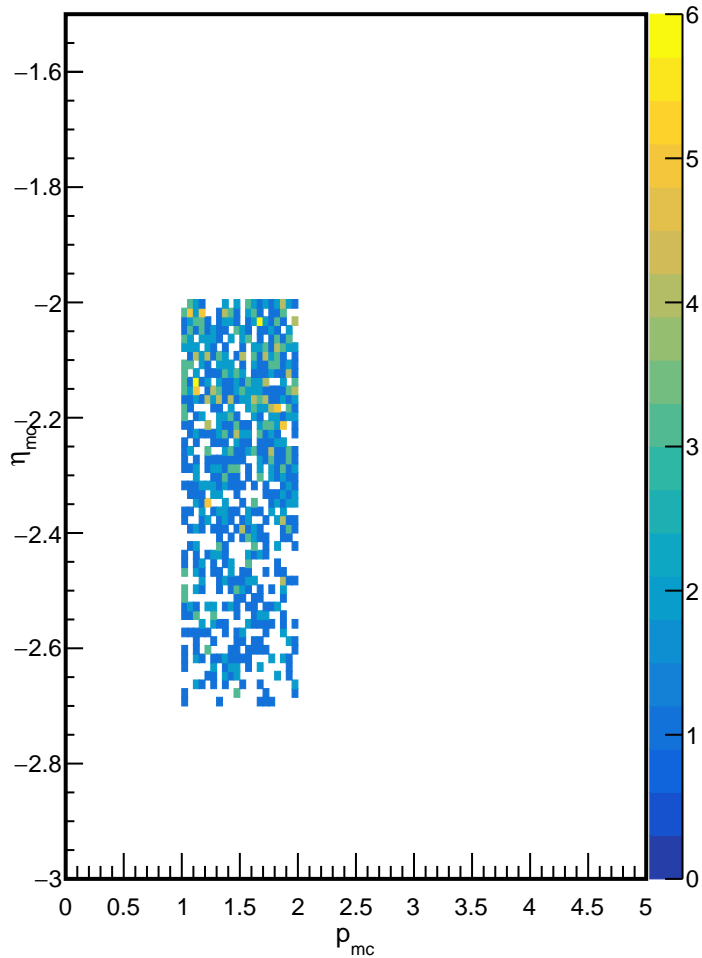
\eta_{\text{mc}} vs p_{\text{mc}}
