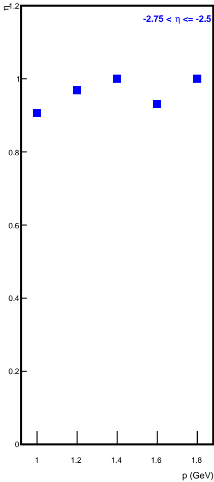
Track Efficiency for -2.75 < \eta \leq -2.5
