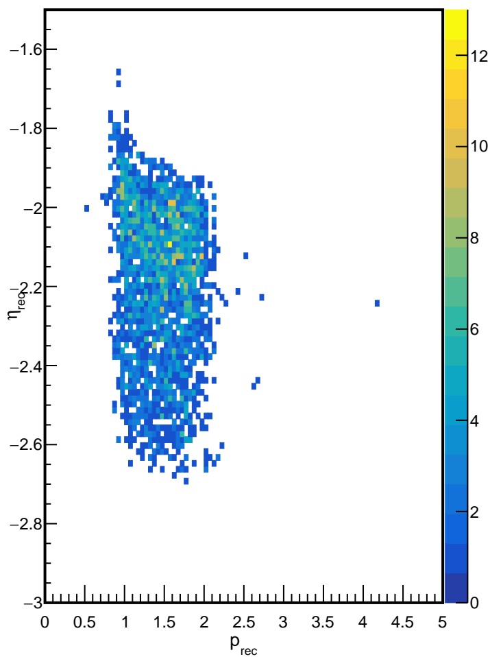
\eta_{\text{rec}} vs p_{\text{rec}}
