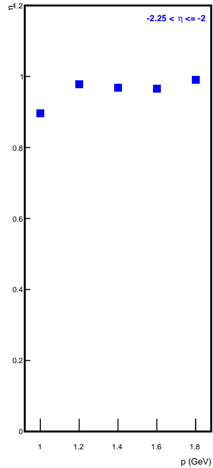
Track Efficiency for -2.25 < \eta \leq -2
