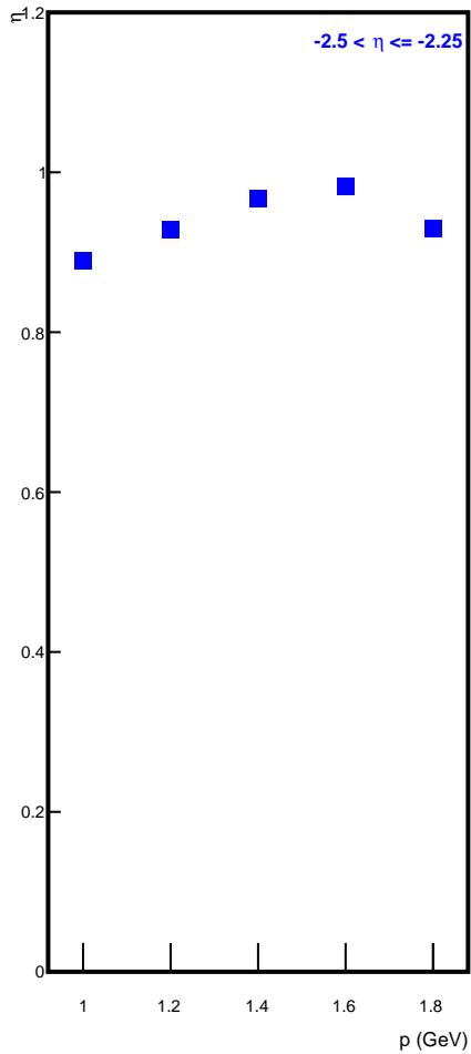
Track Efficiency for -2.5 < \eta \leq -2.25
