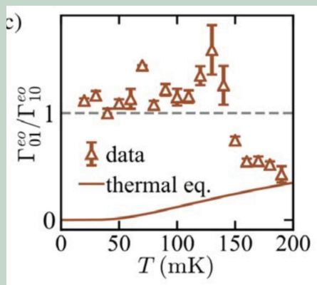
Figure 2: Non-thermal distribution of quasi-particles indicative of cosmic ray and natural sources of radioactivity. | Image reproduced with permission of Brent VanDevender (PNNL).
