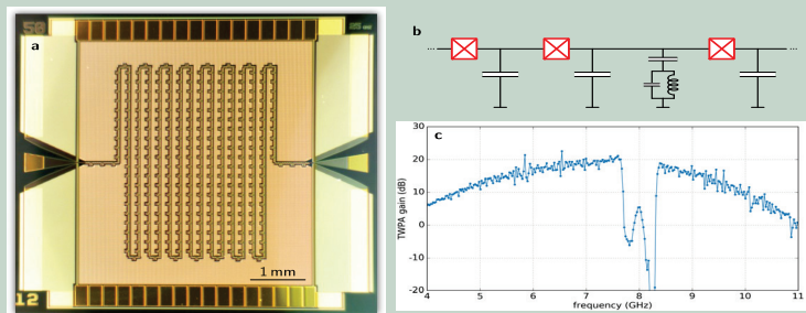
Figure 2: (a) A micrograph of a TWPA showing the path of traveling waves. (b) RF schematic for Josephson TPWAs. (c) Experimentally measured gains of a Josephson TWPA showing wideband performance. | Images reproduced with permission from William Oliver, Massachusetts Institute of Technology, Lincoln Laboratory.
