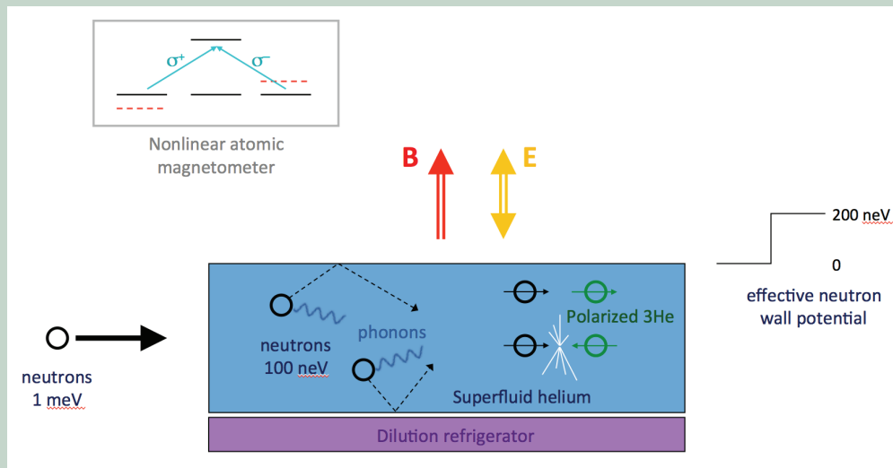
Figure 1: Quantum mechanical effects figure prominently in neutron EDM experiments: (1) Neutrons essentially stop in superfluid helium by transferring all their energy and momentum to the elementary excitations of the macroscopic quantum (superfluid) state. (2) These ultra-cold neutrons exhibit “total internal reflection” from the quantum potential of the container wall. (3) Polarized neutron capture on polarized ^3\text{He} atoms is highly spin dependent; the products of the reaction scintillate in the superfluid, producing an oscillating light signal at the precession frequency. (4) Atomic vapor magnetometers, whose sensitivity is enhanced through quantum coherence, monitor the magnetic field. | Image reproduced with permission from Douglas Beck, University of Illinois, Urbana-Champaign.
