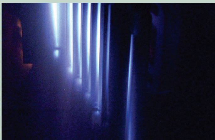
Figure 1: The ionized glow of different ruthenium isotopes upon separation. The electromagnetic ion separator system operates by vaporizing an element, such as ruthenium, into a gas phase, converting the molecules into an ion beam, and then channeling the beam through magnets to separate the different isotopes. | Image reproduced with permission from Brian Egle and David J. Dean, Oak Ridge National Laboratory.
