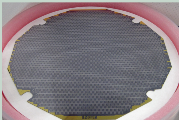
Figure 1: MKIDs on a 135 mm substrate measure small energies deposited in them by charged particles, phonons, and photons. These devices combine high sensitivity with large area coverage. The use of quantum-limited readout amplifiers improves their performance. | Image reproduced by permission of Michael Vissers, NIST. From "The limits of quantum computers," Scientific American 298(3), 62–69, March 2008.
