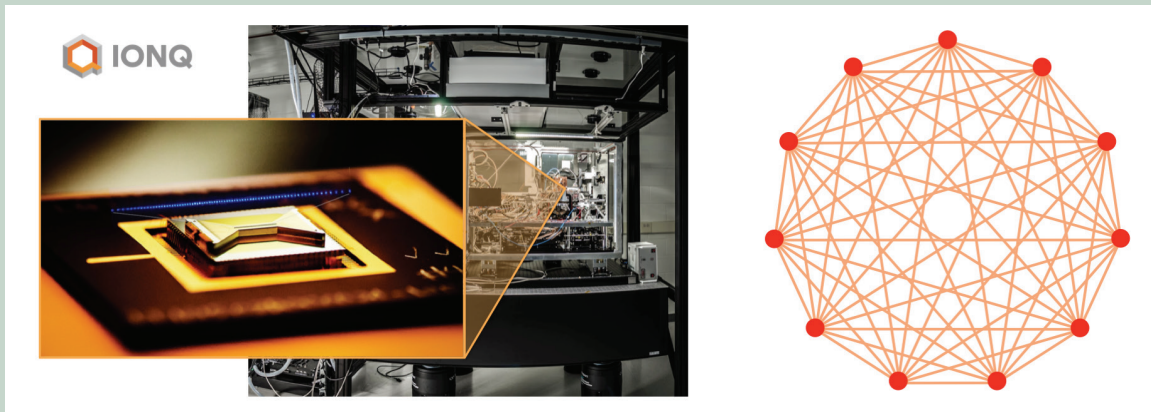
Figure 1: IonQ's trapped-ion digital quantum computer. The left panel shows the quantum computer along with an enlarged view of the ion trap (produced by SNL). The right panel shows the (all-to-all) connectivity map of the 11-qubit QC trapped ion systems that IonQ recently benchmarked. | Images reproduced with permission from IonQ, via Jungsang Kim of Duke University.
