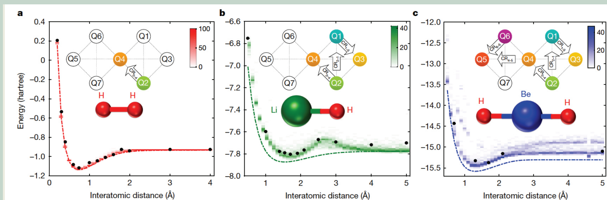
Figure 1: The potential energy between atoms in H_2 , LiH and BeH_2 computed with IBMs quantum systems, compared with the known values. In each panel, the dot-dashed line corresponds to the exact (classically determined) result; the solid, black points are results obtained from the quantum calculations (after measurement and gate error mitigation); and the regions of varying color density correspond to results from 100 classical simulations of the quantum minimization process using the wavefunction ansatz employed for the quantum calculations at each separation distance. | Images reproduced with permission from IBM and Nature Publishing Group. Nature, Hardware-efficient variational quantum eigensolver for small molecules and quantum magnets , A. Kandala et. al., copyright 2017. doi:10.1038/nature23879.
