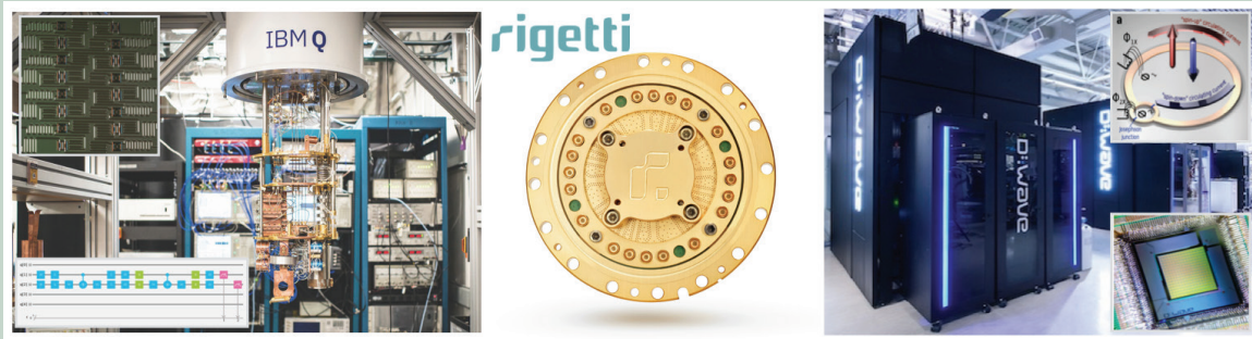
Figure 3: Components of quantum computers produced by IBM (left), Rigetti (center) and D-Wave (right). The upper inset of left panel is IBM’s 16 qubit chip and the lower inset is a quantum circuit implemented through IBM’s “qiskit” web-interface. The upper inset of the right panel is D-Wave’s superconducting loop qubit and the lower inset is its 2000 qubit annealing processor. | Images reproduced with permission from Nature Publishing Group. Nature, Hardware efficient variational quantum eigensolver for small molecules and quantum magnets, A. Kandala et al., copyright 2017.
