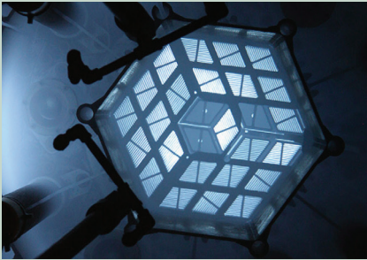
Figure 3: The MIT reactor being used to produce ^{64}\text{Cu} for use in controlled background experiments to measure the impact of radioactivity on quasi-particle distributions in superconducting qubits. | Image reproduced with permission from Joseph Formaggio, MIT.
