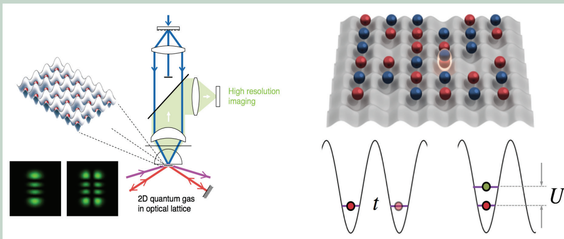
Figure 2: Elements of an optically trapped cold-atom analogue quantum simulator (left panel) and elements in simulating the Fermi Hubbard model. | Images reproduced with permission from Markus Greiner, Harvard University
