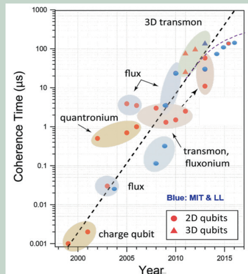
Figure 1: Quantum "Moore's Law" for superconducting qubit coherence times, T_2 . | Image reproduced from Oliver and Welander, Materials in superconducting quantum bits , MRS Bulletin 38, 816-825 (2013), copyright by Materials Research Society. Updated by Brent VanDevender (2019). Reproduced with permission of Brent VanDevender (PNNL) and Will Oliver (MIT).
