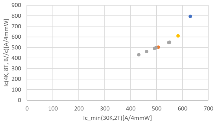
1.9um REBCO tapes
