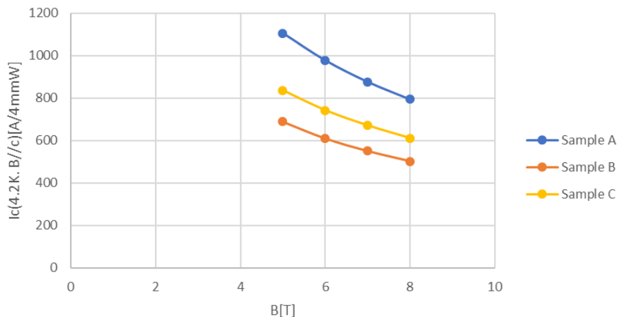
1.9um REBCO film 4K-B
